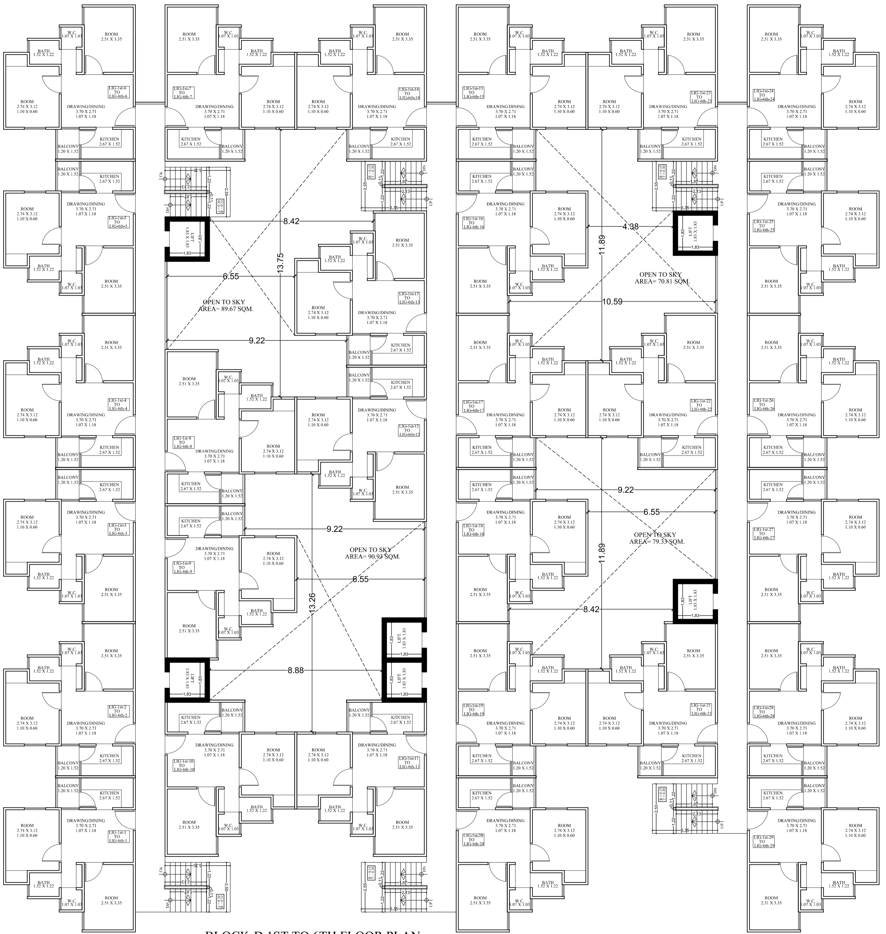
BLOCK-D 1ST TO 6TH FLOOR PLAN
